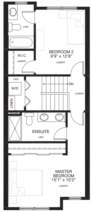
UPPER FLOOR Finished Area: 628 Sq.Ft.
