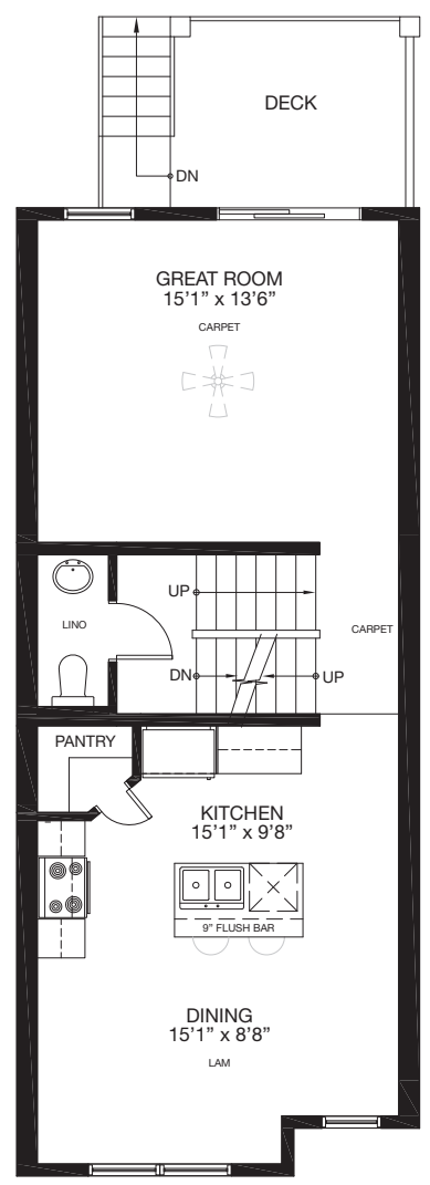
MAIN FLOOR Finished Area: 638 Sq.Ft.
