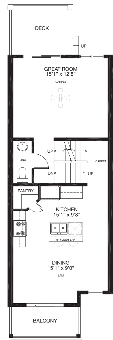
MAIN FLOOR Finished Area: 630 Sq.Ft.
