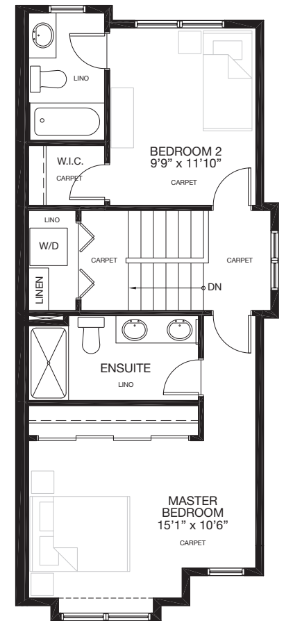
UPPER FLOOR Finished Area: 638 Sq.Ft.
